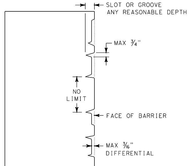
GAPS, SLOTS, GROOVES OR JOINTS
