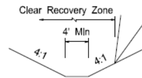
Preferred Trapezoidal Channel Section If Within CRZ
