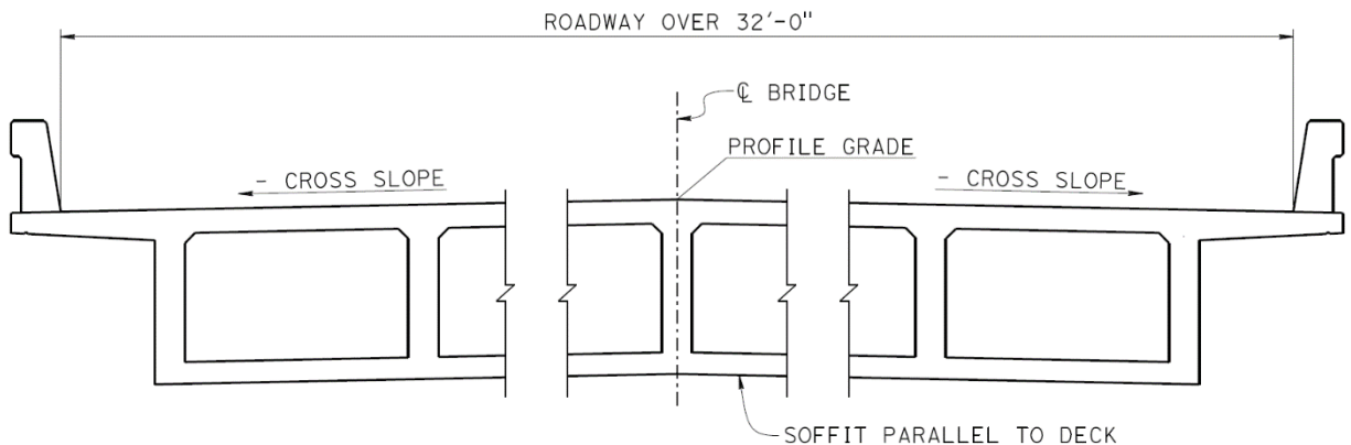
Figure 8.2.2 Box Girder Parallel Soffit
