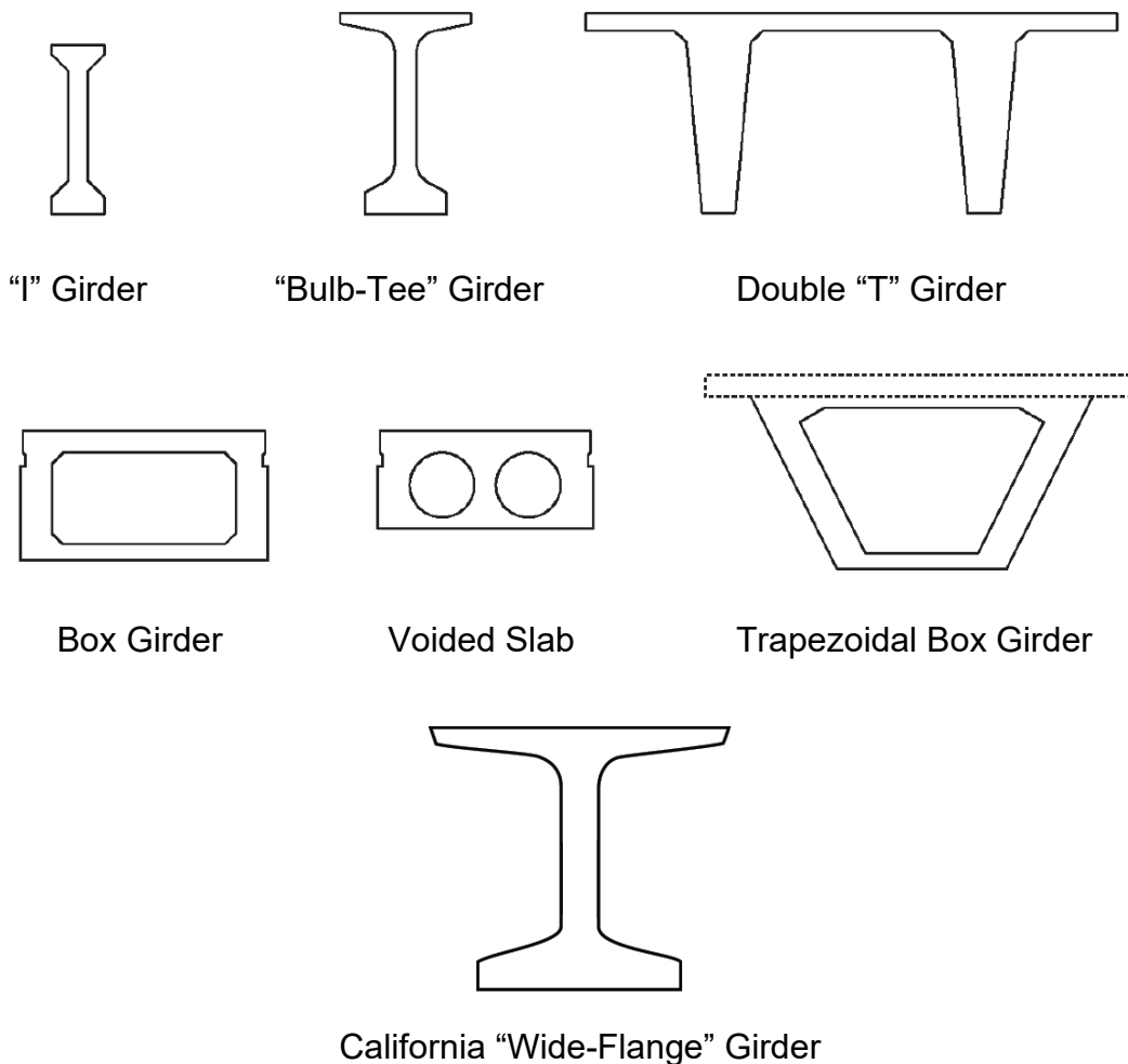
Figure 8.4.1 Standard Precast Girders
