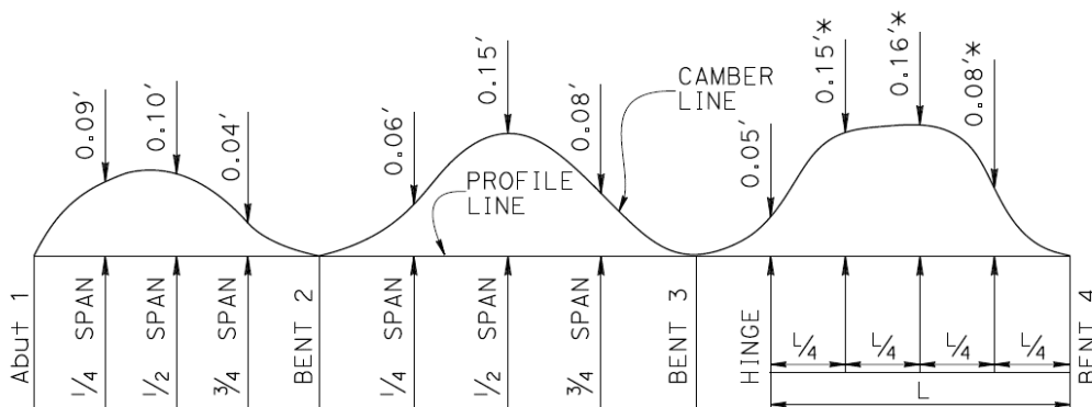
Figure 9.2.1 Three-Span Camber Diagram
