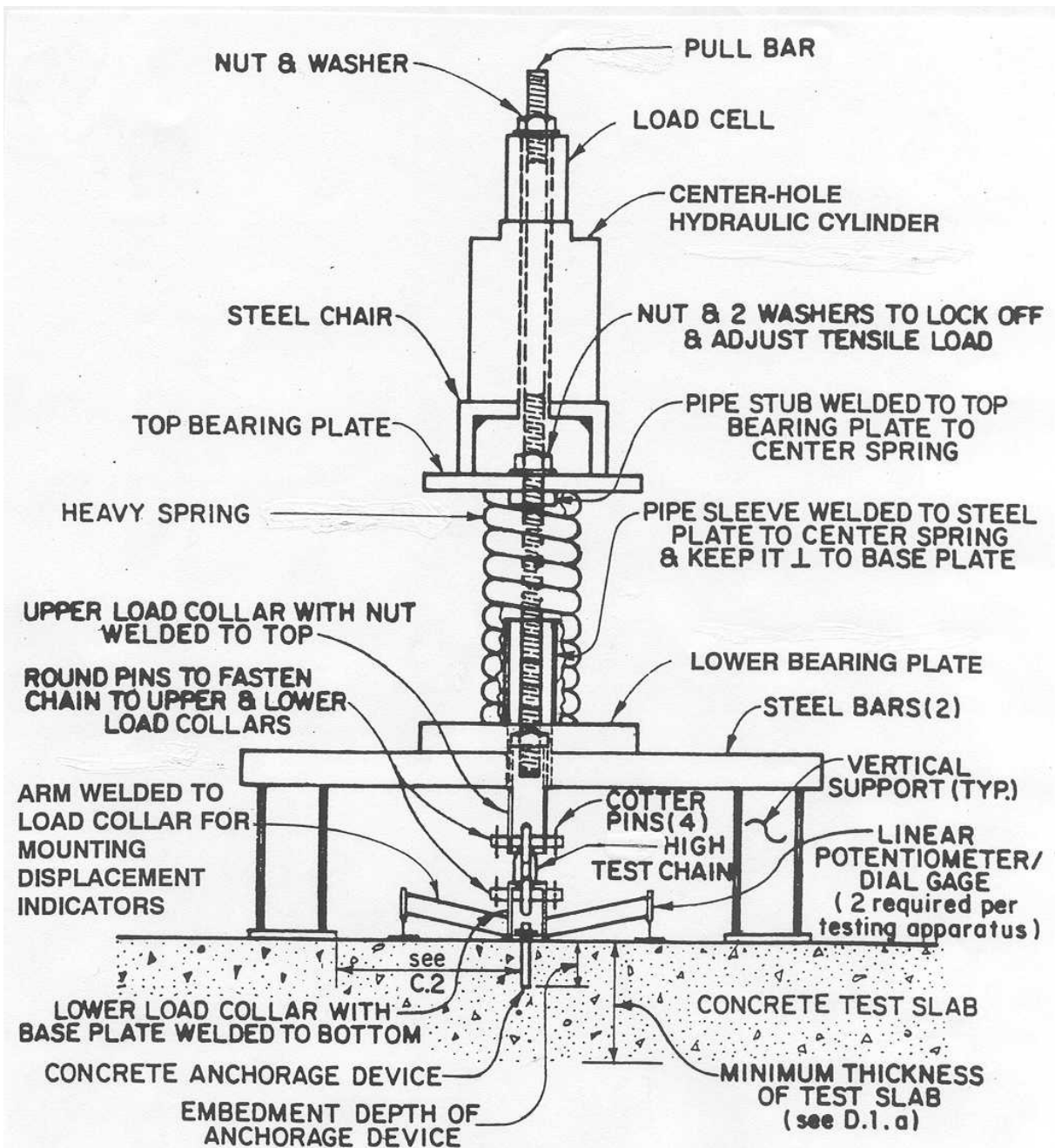
FIGURE 1. EXAMPLE OF A SUITABLE CREEP TESTING APPARATUS
