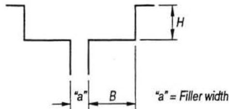
Blockout Dimensions
