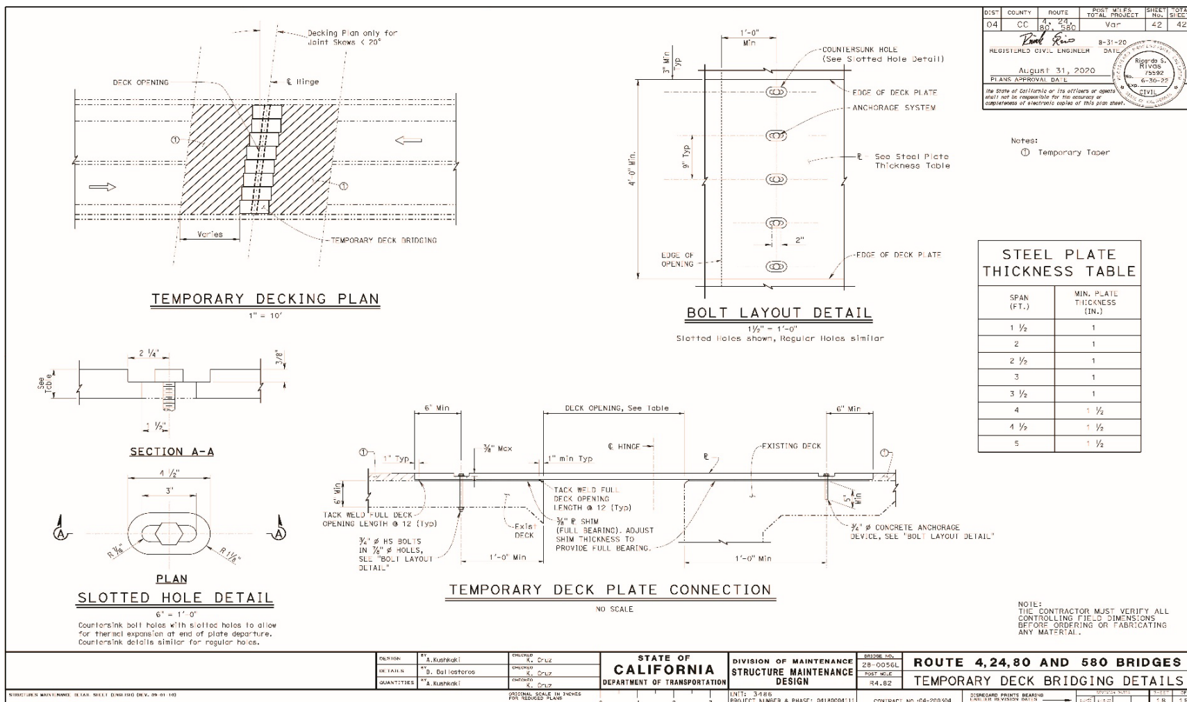
Figure 1. Sample Temporary Decking Plan
