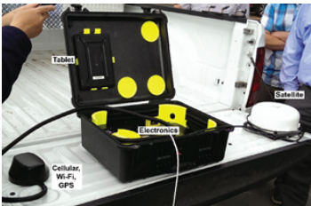
Image 1: Responder Architecture
