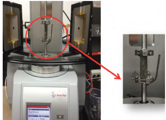
Figure 1: Testing fine aggregate matrix specimens in a dynamic shear rheometer
