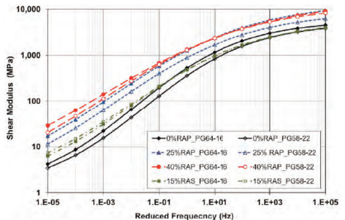
Figure 2: Shear modulus curves of fine aggregate matrix mixes containing various percentages of RAP and RAS
