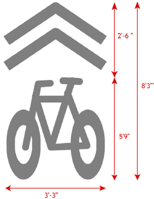
Figure 11. Recommended Modified Bike-and-Chevron
