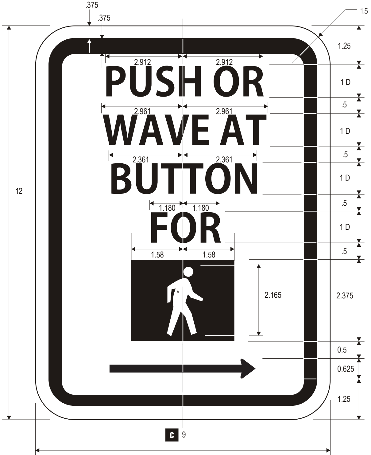
R10-3j (CA) PEDESTRIAN TRAFFIC SIGNAL
